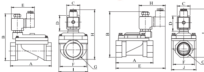
Dimensions (mm)
